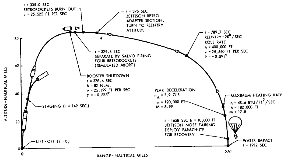
Figure 40.—McDonnell's proposed sequence of events for the first Gemini mission. (McDonnell, "Project Gemini Mission Plan, Spaccraft No. 1," Sept. 14, 1962, p. 7.)
