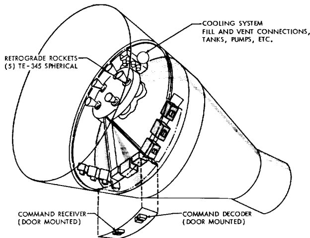
Figure 7.—The adapter section of McDonnell's proposed two-man Mercury spacecraft. (McDonnell Report, "Manned Spacecraft—Advanced Versions," July 27-28, 1961, part 4, "Two Man MK II Spacecraft," unpagged.)
