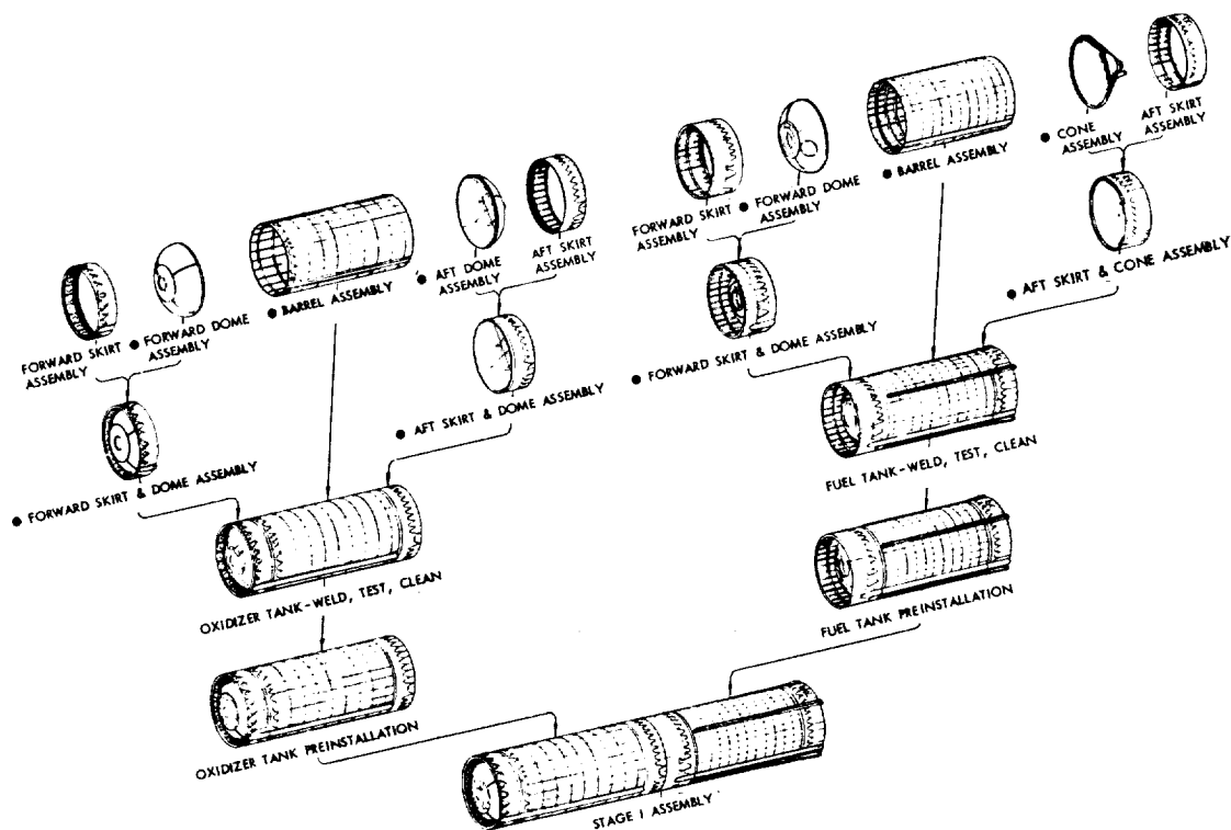
Figure 49(A).—Procedure for assembling fuel and oxidizer tanks for stage I of the Gemini launch vehicle. (Martin Photo 8B65793, undated.)
