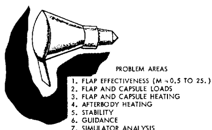
Figure 2.—One version of the "lifting" Mercury capsule being considered in 1960 for a flight-test program between the end of Mercury and the start of a manned circumlunar program. (STG, "Guidelines for Advanced Manned Space Vehicle Program," June 1960, p. 53)
