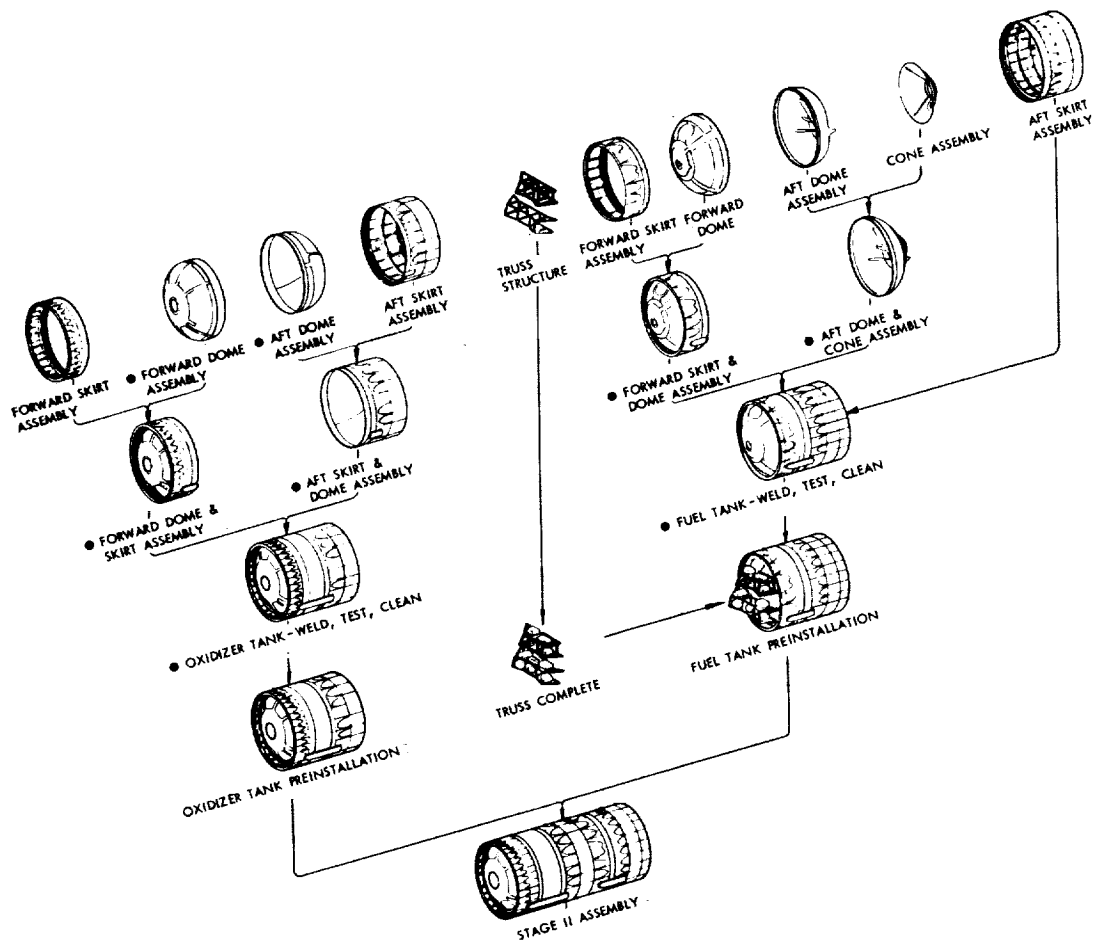
Figure 49 (B).—Procedure for assembling fuel and oxidizer tanks for stage II of the Gemini launch vehicle. (Martin Photo 8B65794, undated.)
