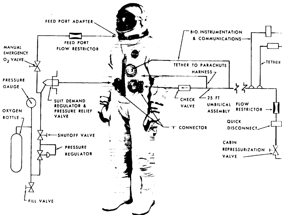
Figure 81.—Diagram of the Gemini G4C extravehicular suit. (NASA Photo S-65-4858, May 1965.)
