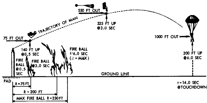
Figure 34.—The "off-the-pad" escape mode for an aborted Gemini mission. (Charts presented by K. Hecht, "Project Gemini Familiarization Briefing," July 9-10, 1962, unpagged.)
