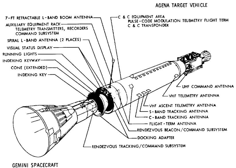
Figure 92.—Location of command and communications system equipment on the Agena target vehicle. (Lockheed Photo NP-2-23, June 1,
