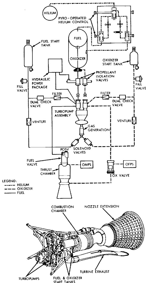
Figure 50.—Schematic and drawing of the primary propulsion system of the Gemini Agena target vehicle. (Lockheed, Gemini Agena Target Press Handbook, LMSC-A766871, Feb. 15, 1966, pp. 4-19, 4-20.)
