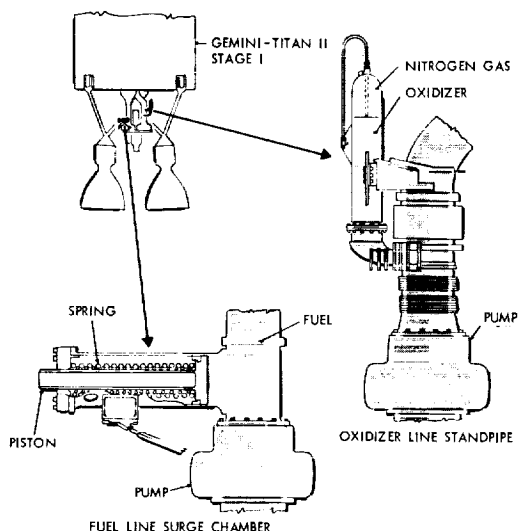
Figure 51.—POGO suppression equipment proved out in the Titan II development program. (Martin Photo 8B65766, undated.)
