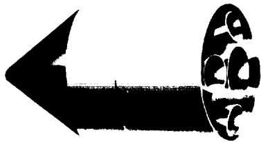
CIRCUMLUNAR
