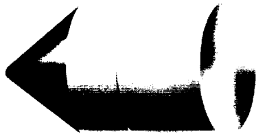
EARTH ORBIT
